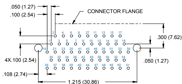
51 PIN
