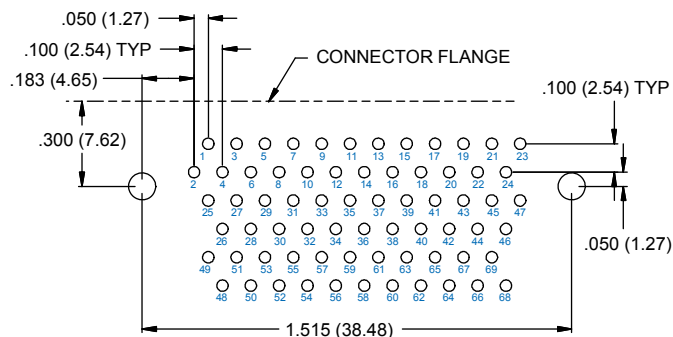
69 PIN
