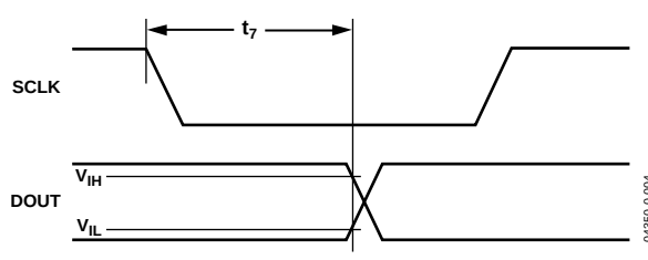
Figure 4. Hold Time after SCLK Falling Edge
