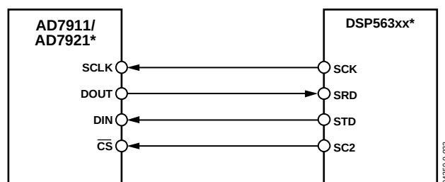
Figure 34. Interfacing to the DSP563xx
