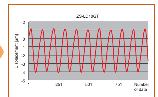
Inspection of Disk Play on HDD Motor Rotating Plate
