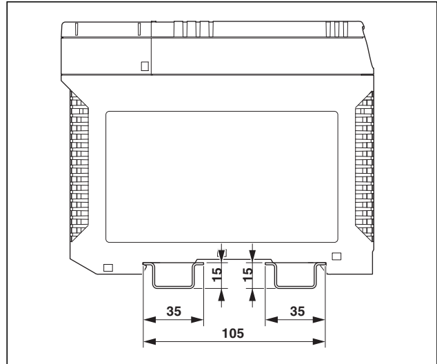
Figure 49 Dimensional drawing with NS 35/15
