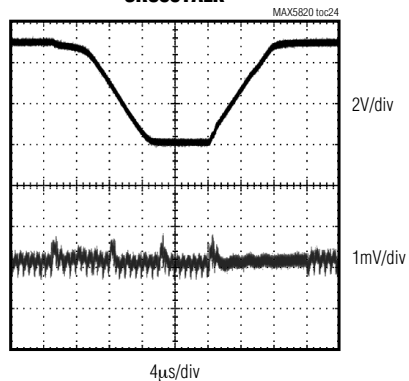
CROSSTALK
