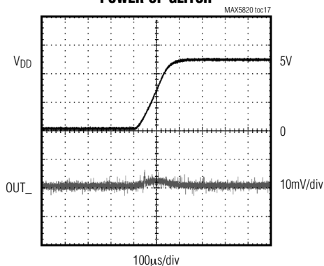
POWER-UP GLITCH
