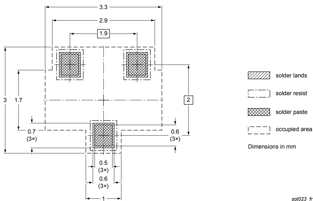
Fig. 14. Reflow soldering footprint for TO-236AB (SOT23)
