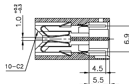
SECT "A"-"A"
