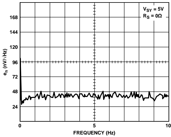
Figure 44. Voltage Noise Density at 5 V from 0 Hz to 10 Hz
