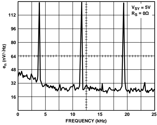
Figure 43. Voltage Noise Density at 5 V from 0 Hz to 25 kHz
