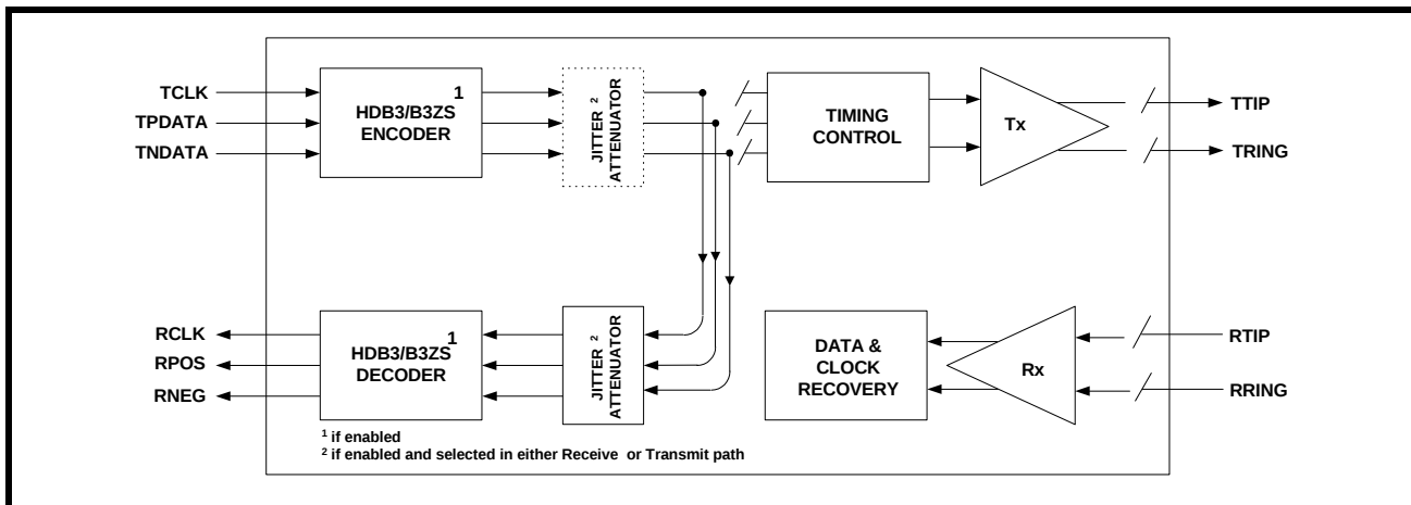
FIGURE 27. DIGITAL LOOPBACK
