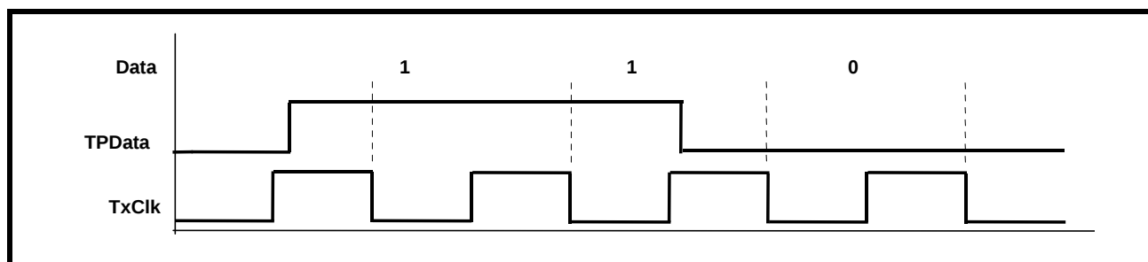
FIGURE 12. SINGLE-RAIL OR NRZ DATA FORMAT (ENCODER AND DECODER ARE ENABLED)
