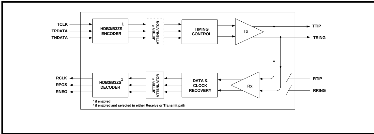
FIGURE 26. ANALOG LOOPBACK
