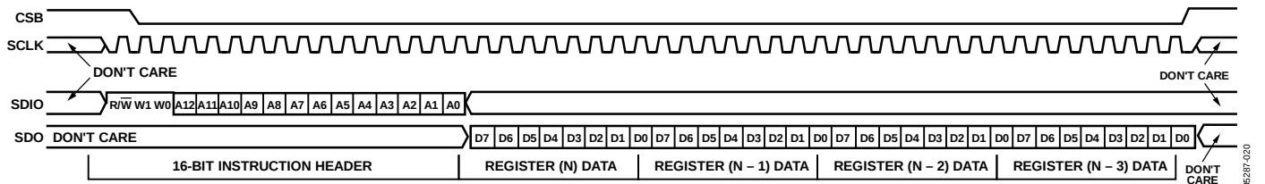
Figure 33. Serial Control Port Read—MSB First, 16-Bit Instruction, 4 Bytes of Data
