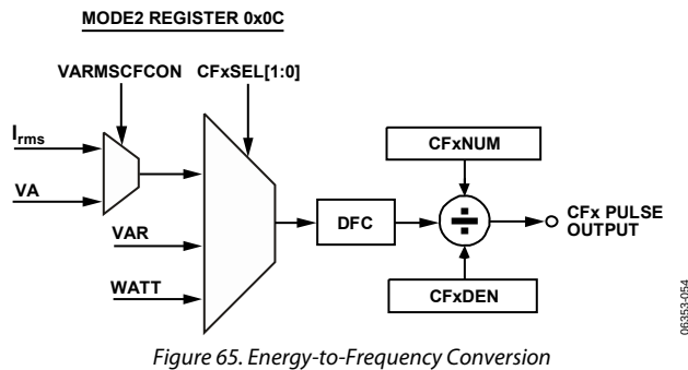
Figure 65. Energy-to-Frequency Conversion
