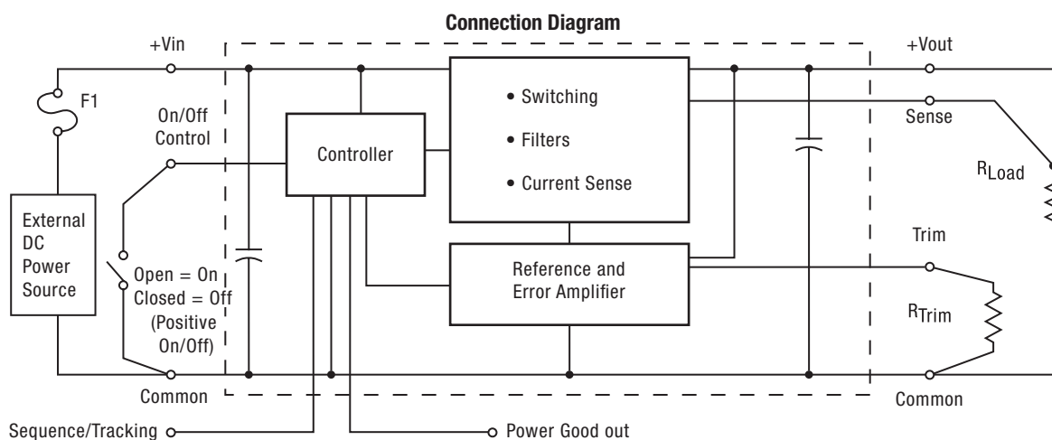
Figure 1. OKL2-T/6-W12
