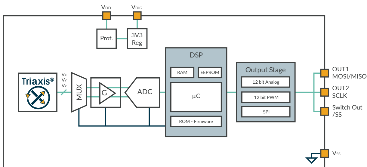
Figure 1 – Block Diagram
