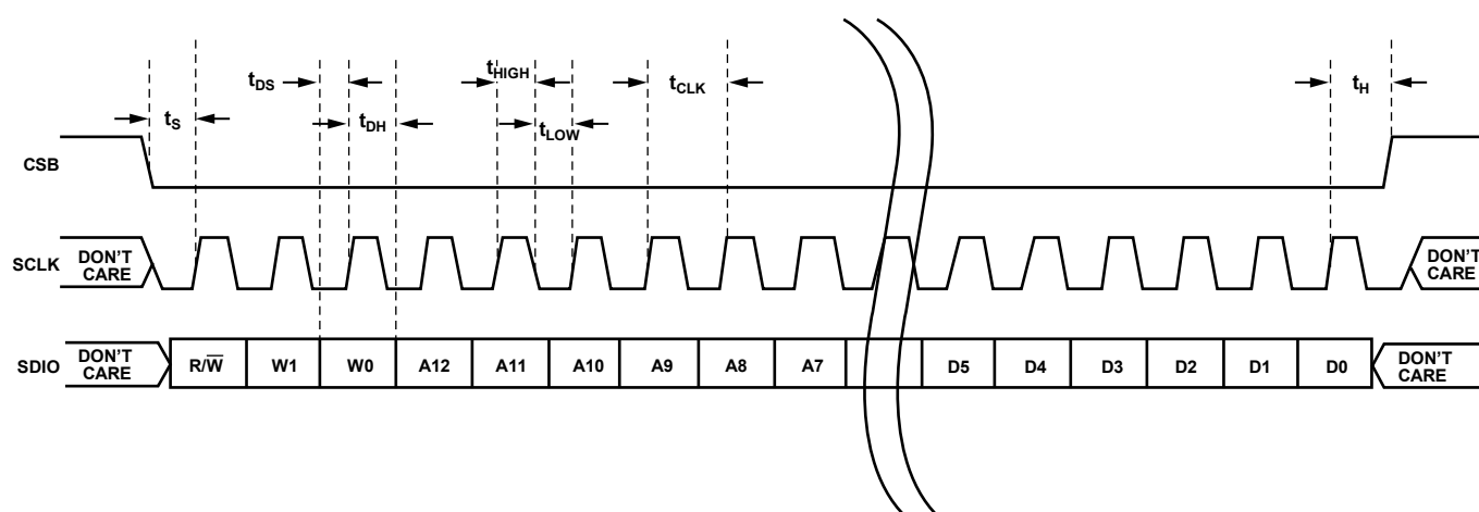
Figure 58. Serial Port Interface Timing Diagram
