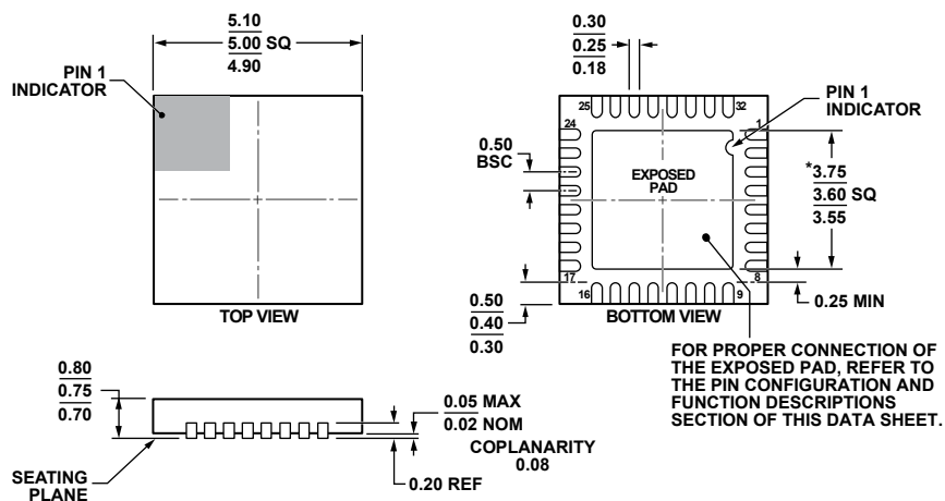
Figure 59. 32-Lead Lead Frame Chip Scale Package [LFCSP_WQ] 5 mm × 5 mm Body, Very Thin Quad (CP-32-12) Dimensions shown in millimeters
