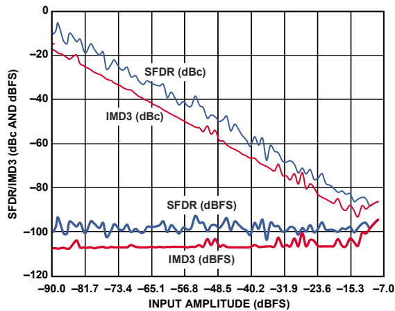
Figure 11. AD9642-170 Two-Tone SFDR/IMD3 vs. Input Amplitude ( A_{IN} ) with f_{IN1} = 184.12 MHz, f_{IN2} = 187.12 MHz, f_s = 170 MSPS
