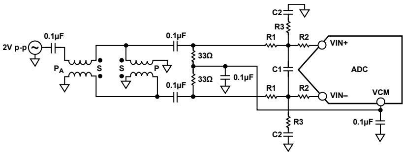
Figure 50. Differential Double Balun Input Configuration
