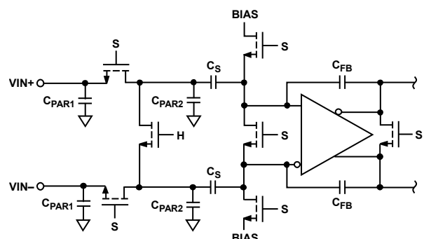
Figure 46. Switched-Capacitor Input
