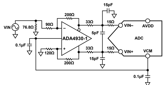
Figure 47. Differential Input Configuration Using the ADA4930-1
