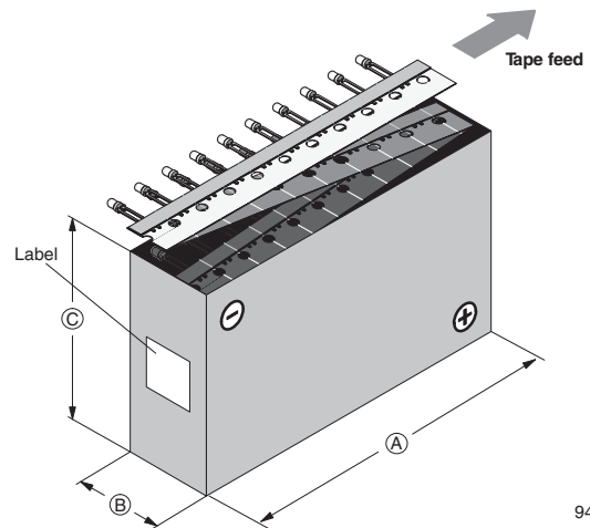
Fig. 41 - Tape Direction
