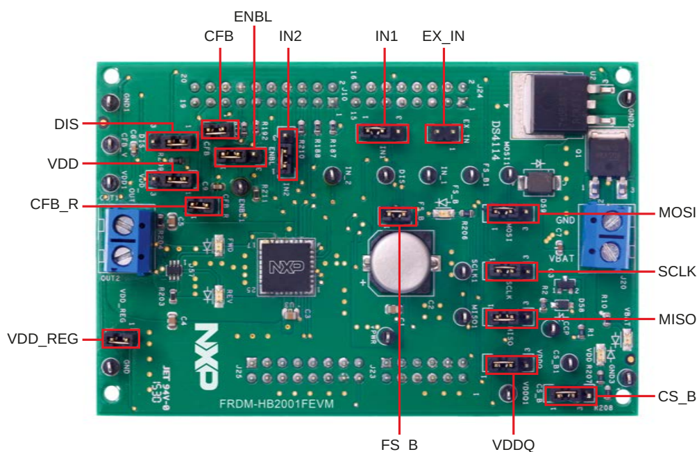
Figure 7. Jumper definitions
