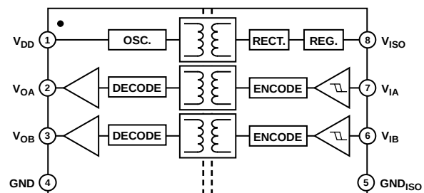
Figure 3. ADuM5242
