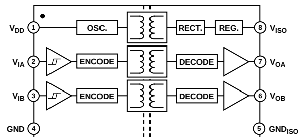
Figure 1. ADuM5240
