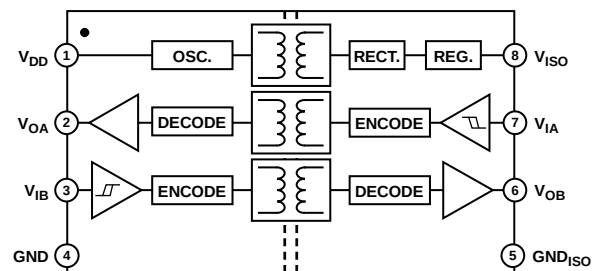
Figure 2. ADuM5241
