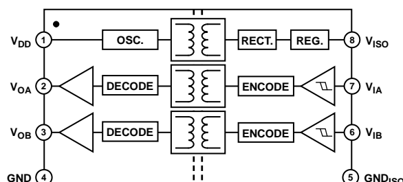
Figure 3. ADuM5242
