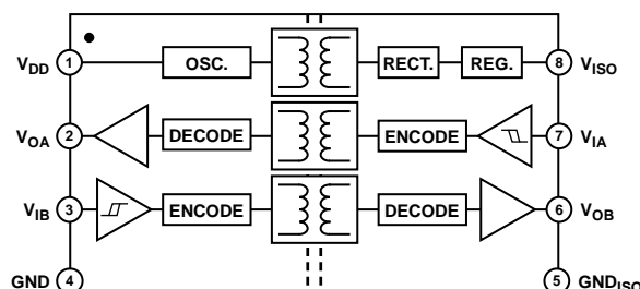
Figure 2. ADuM5241
