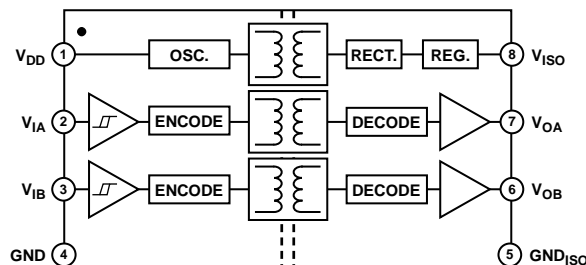
Figure 1. ADuM5240
