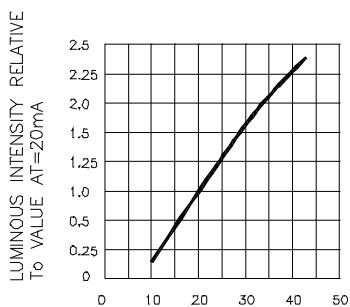
If-FORWARD CURRENT-mA
