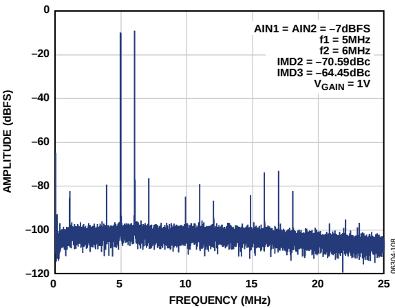
Figure 38. Typical IMD3 and IMD2 Performance
