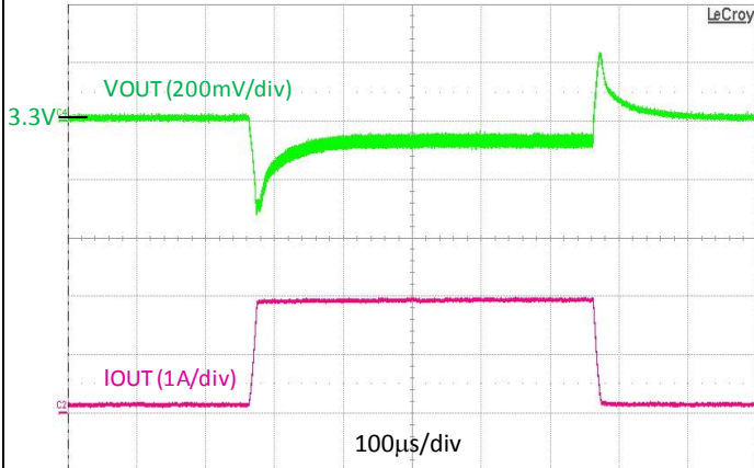
Figure 35. Load Transient, 150-2000 mA, 10 µs Edge, V_{IN}=3.0\text{ V} , V_{OUT}=3.3\text{ V}
