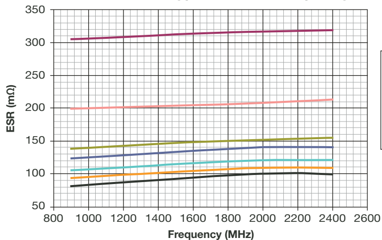
Accu-P® 0805 Typical ESR vs Frequency
