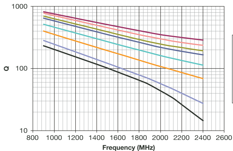
Accu-P® 0805 Typical Q vs Frequency
