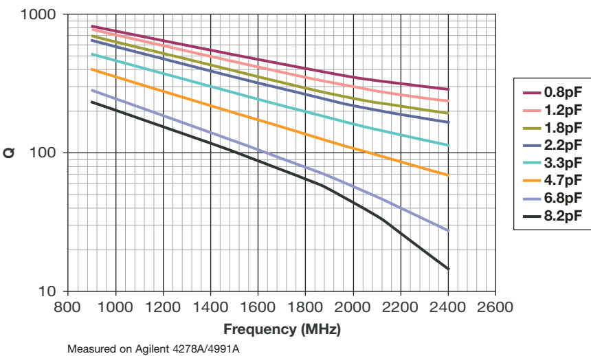
Accu-P ® 0805 Typical Q vs Frequency
