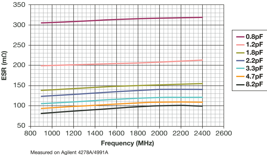
Accu-P ® 0805 Typical ESR vs Frequency
