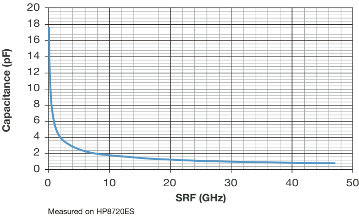
Accu-P ® 0805 Typical SRF vs Capacitance
