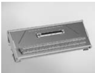
ADAM-39100 100-pin DIN-rail SCSI Wiring Board
