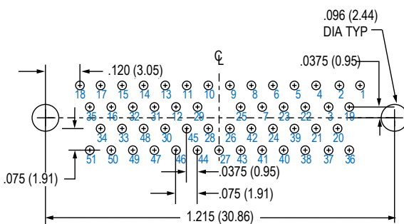
51 SOCKET
