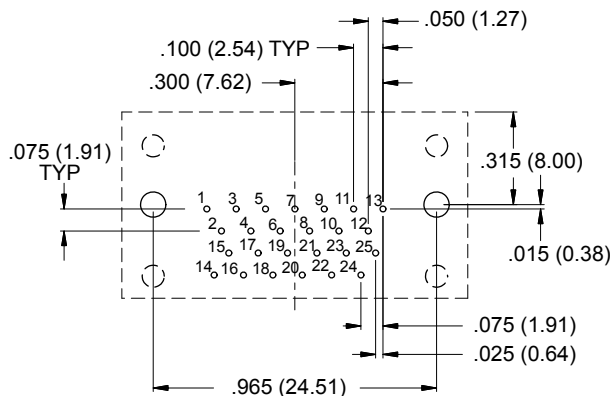
25 PIN
