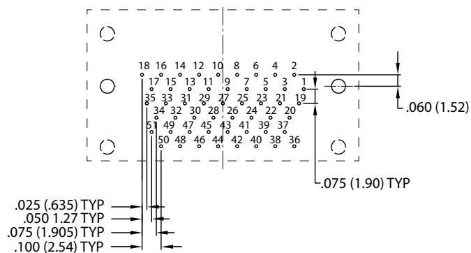
51 SOCKET
