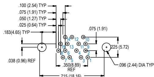
15 PIN
