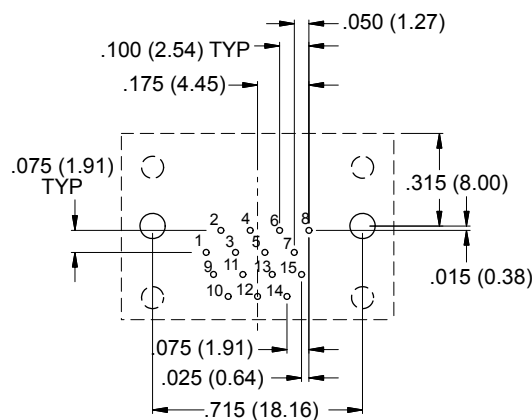
15 PIN
