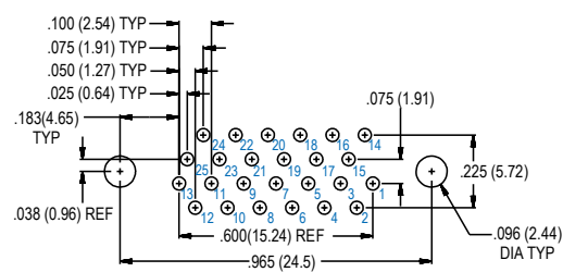
25 PIN
