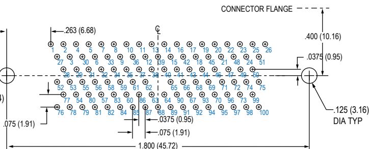
100 PIN
