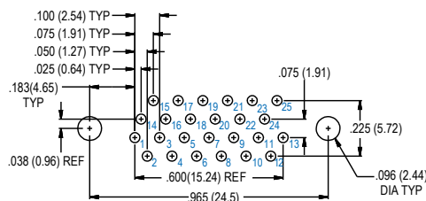
25 SOCKET
