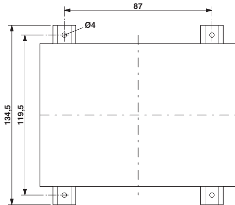
Dimensional drawing
