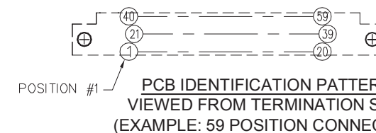
PIN IDENTIFICATION PATTERN VIEWED FROM TERMINATION SIDE (EXAMPLE: 59 POSITION CONNECTOR)
