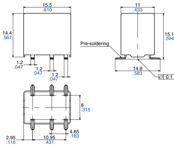
External dimensions
