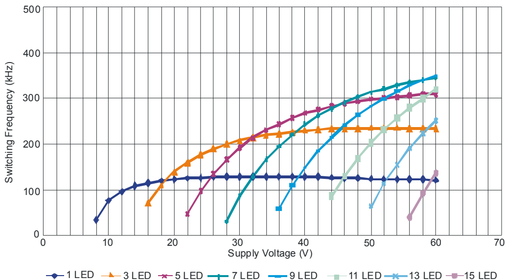
ZXLD1362 Switching Frequency L = 100\mu\text{H}
