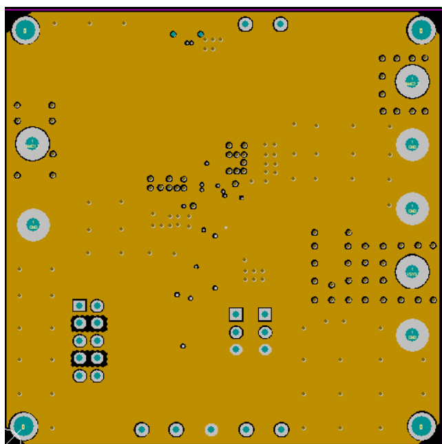
Figure 3—Middle Layer1
