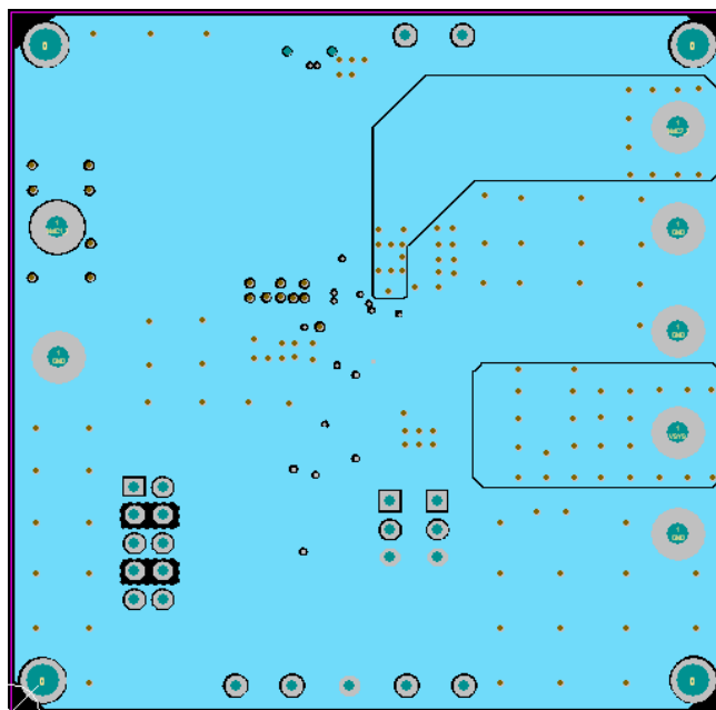
Figure 4—Middle Layer2
