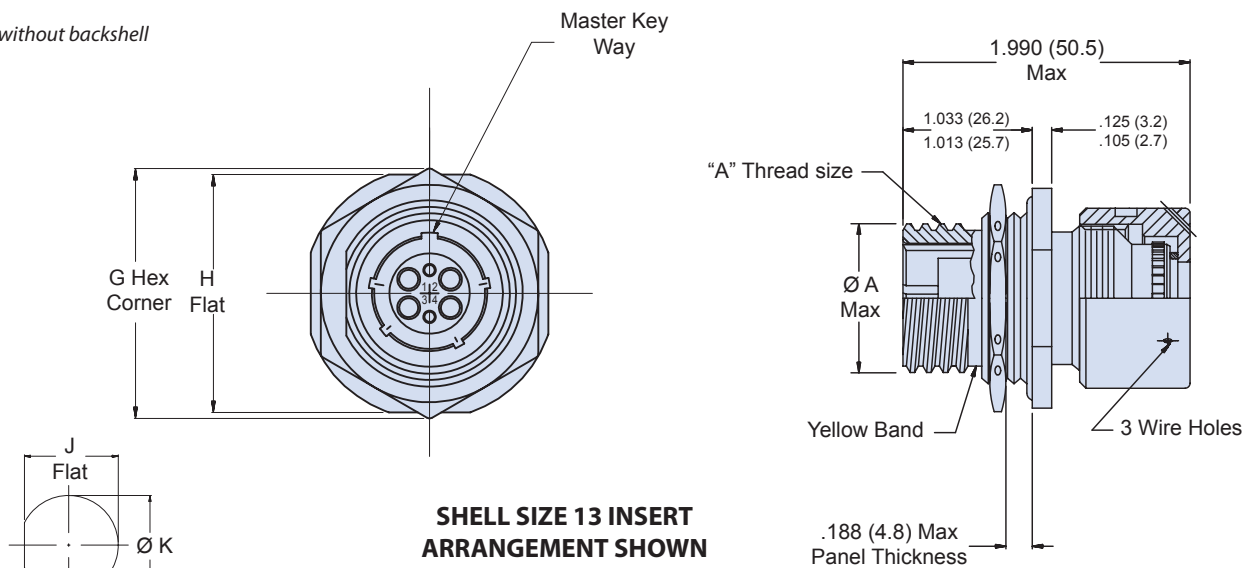
04 - JAM NUT MOUNT RECEPTACLE WITHOUT BACKSHELL M28876/11 • 180-040 (-04)
