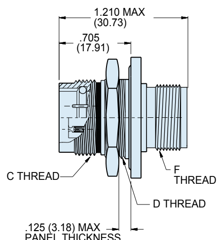
RECEPTACLE WITH ACCESSORY THREAD 802-011
