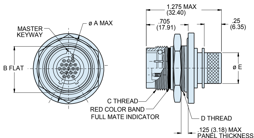
RECEPTACLE WITH INTEGRAL BAND PLATFORM 802-010
