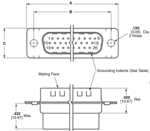
Plug
