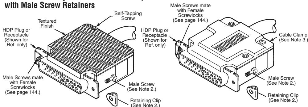
Shell Size 1 & 2
