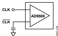
Figure 37. Typical 2.5 V or 3.3 V CMOS Configurations for Short Trace Lengths
