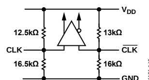
Figure 43. AD9508 Differential Input Stage
