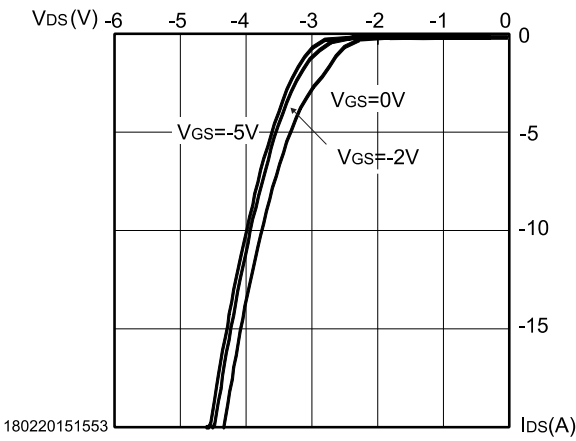
Figure 16: Body diode characteristics ( T_J = -50 °C)
