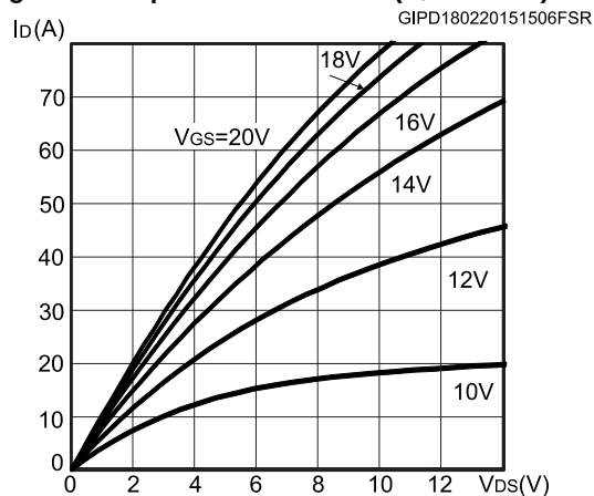
Figure 6: Output characteristics ( T_J = 200\text{ }^{\circ}\text{C} )
