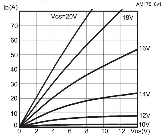
Figure 4: Output characteristics ( T_J = 25\text{ }^{\circ}\text{C} )
