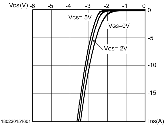
Figure 18: Body diode characteristics ( T_J = 150 °C)
