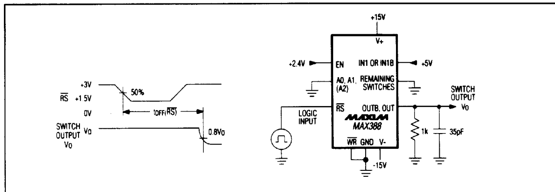
Figure 6. Reset Turn-Off Time ( t_{OFF}(\overline{RS}) )
