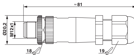
M12 x 1 plug, straight
