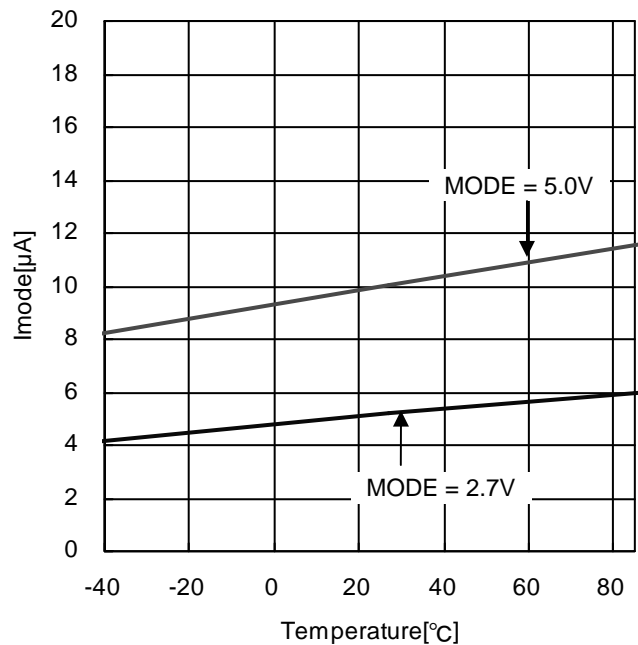
Figure 11. Mode Input Current - Temperature
