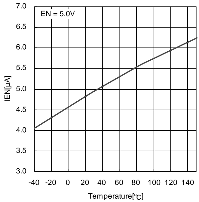
Figure 21. EN Input Current - Temperature
