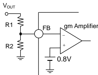
Figure 51. Feedback Resistor Circuit
