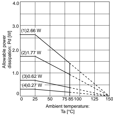
Figure 57. Thermal Derating Characteristics (VQFN016V3030)
