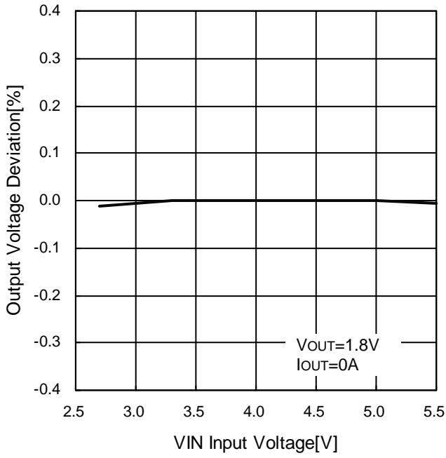
Figure 37. VOUT Line Regulation (VOUT = 1.8V)
