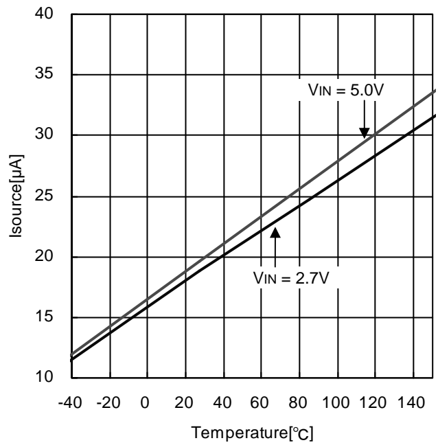
Figure 9. ITH Source Current - Temperature
