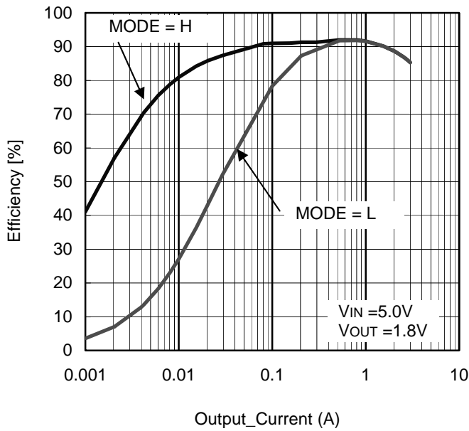
Figure 22. Efficiency – Output Current (VIN=5V, VOUT=1.8V, L=1.5μH)
