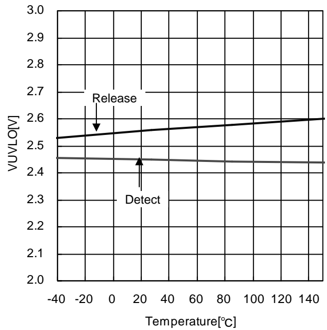
Figure 19. UVLO Threshold - Temperature
