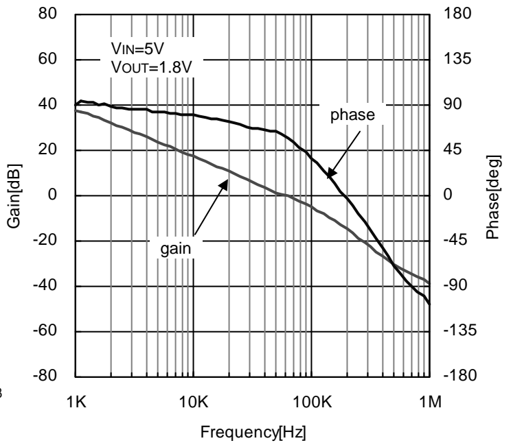
Figure 25. Loop Response (VIN=5V, VOUT=1.8V, IOUT=1A, L=1.5μH, COUT=Ceramic44μF)
