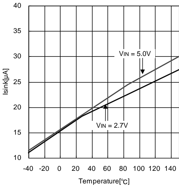
Figure 8. ITH Sink Current - Temperature
