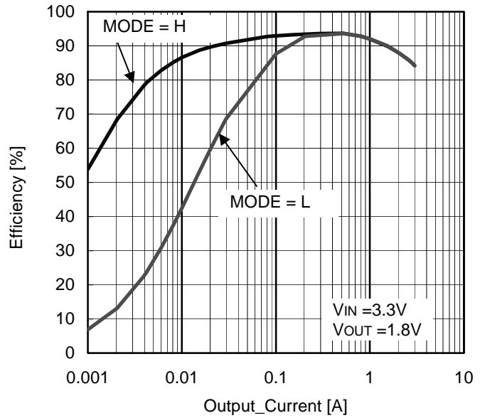
Figure 23. Efficiency – Output Current (VIN=3.3V, VOUT=1.8V, L=1.5μH)
