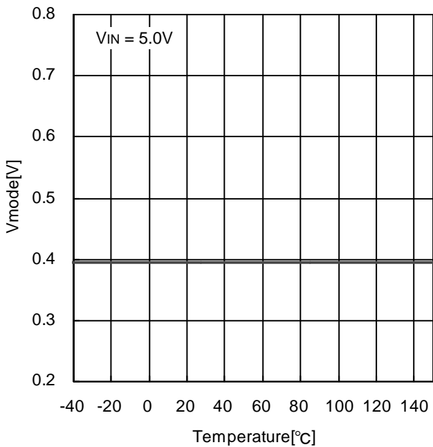
Figure 10. Mode Threshold - Temperature
