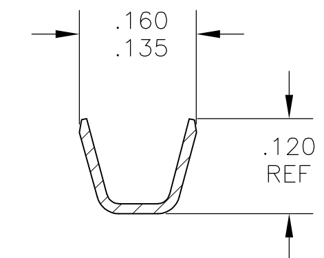
SECTION Y-Y
