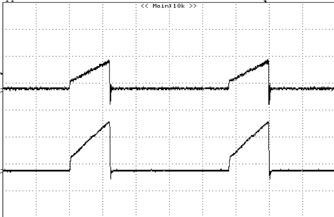
Figure 25: Typical transient response to step load change at 5A/\mu S from 25% to 75% of I_{o, max} at 12Vin, 3.3V out (Cout = 1uF ceramic, 10uF tantalum) Top: 100mV/div, 50uS/div, Bottom: 20A/div, 50uS/div
