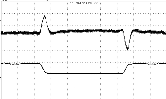
Figure 25: Typical transient response to step load change at 5A/\mu S from 25% to 75% of I_{o, max} at 12Vin, 3.3V out (Cout = 1uF ceramic, 10uF tantalum) Top: 100mV/div, 50uS/div, Bottom: 20A/div, 50uS/div
