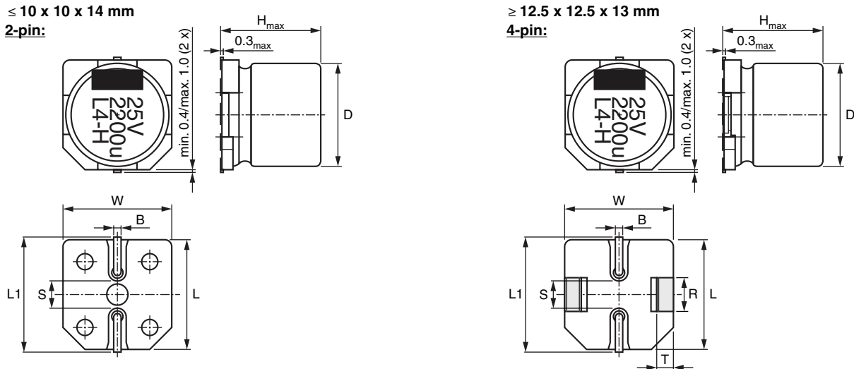
Fig.2 Dimensional outline
