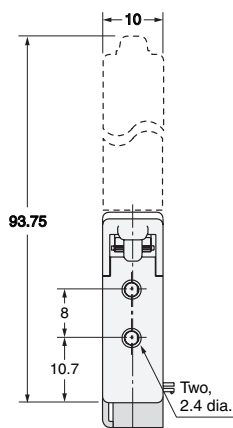
Mounting Holes
