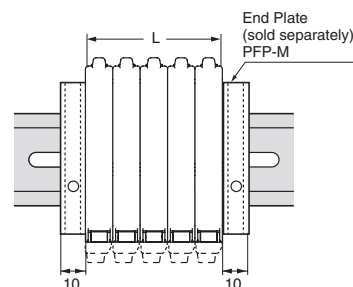
Multiple connection diagram
