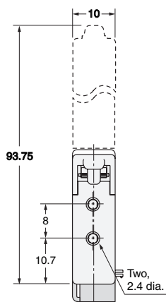
Mounting Holes
