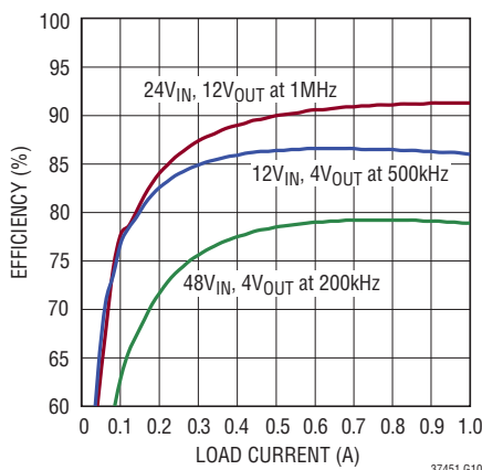
Buck Efficiency
