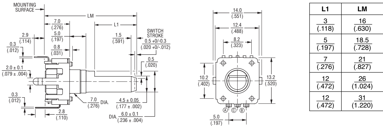
PEL12T-4xxxF-S1024 (Horizontal Mount w/Triple LED & Switch, Flatted Shaft)
