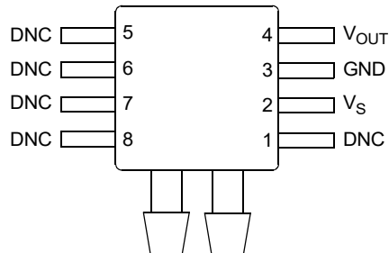
Figure 2. Full device pinout (top view)
