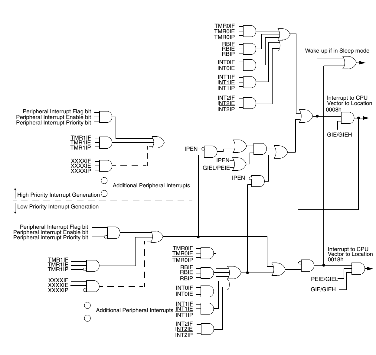
FIGURE 8-1: INTERRUPT LOGIC
