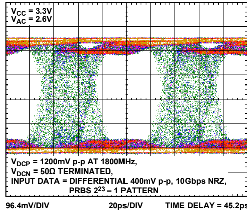
Figure 33. Output Eye Diagram Continuous Snapshot for 10 Gbps Input
